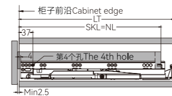
外置抽屉 Standard drawer
