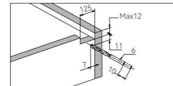
抽屉尺寸和钻孔(mm) Drawer size and drilling
