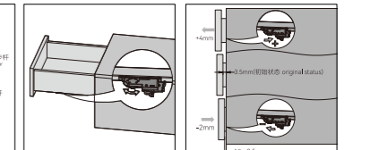
抽屉面板缝隙调节(+4~-2mm) Front panel gap adjustment(+4~-2mm)
