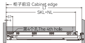
外置抽屉 Standard drawer
