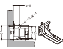
B(塑胶连接件)(Plastic bracket)
