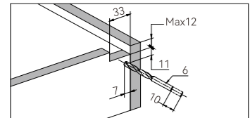
抽屉尺寸和钻孔(mm) Drawer size and drilling
